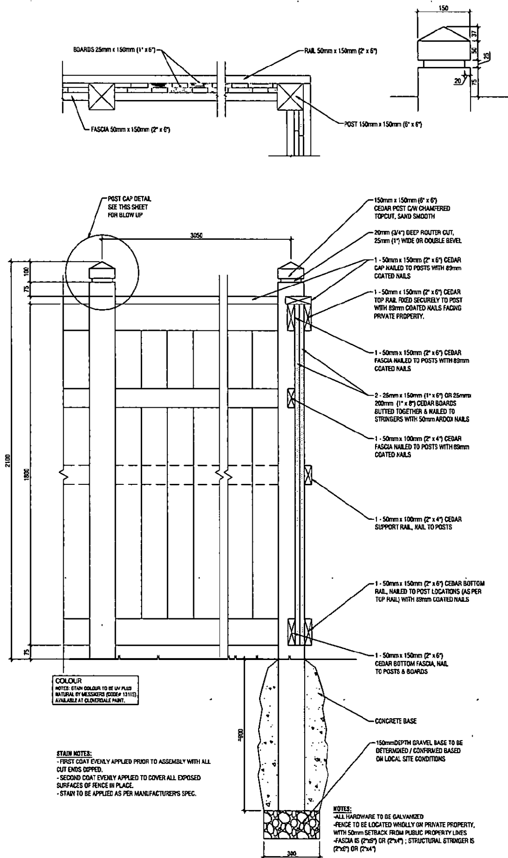
1.8M HT. CEDAR OVERLAP WOOD SCREEN FENCE N.T.B
