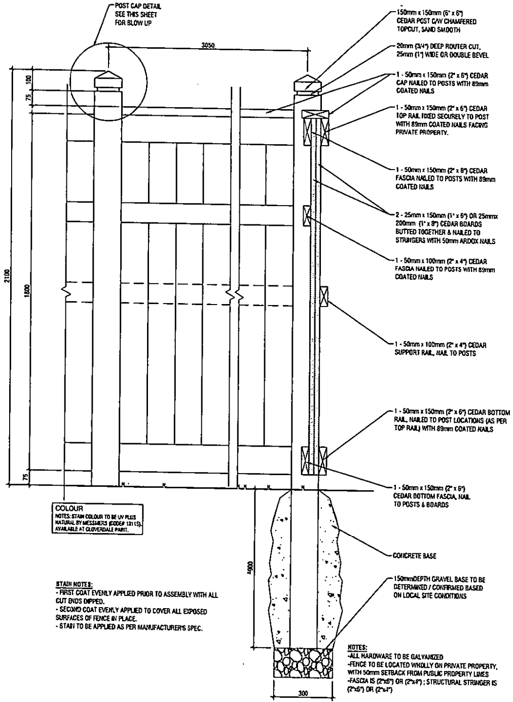
1.8M HT. CEDAR OVERLAP WOOD SCREEN FENCE N.T.S.
